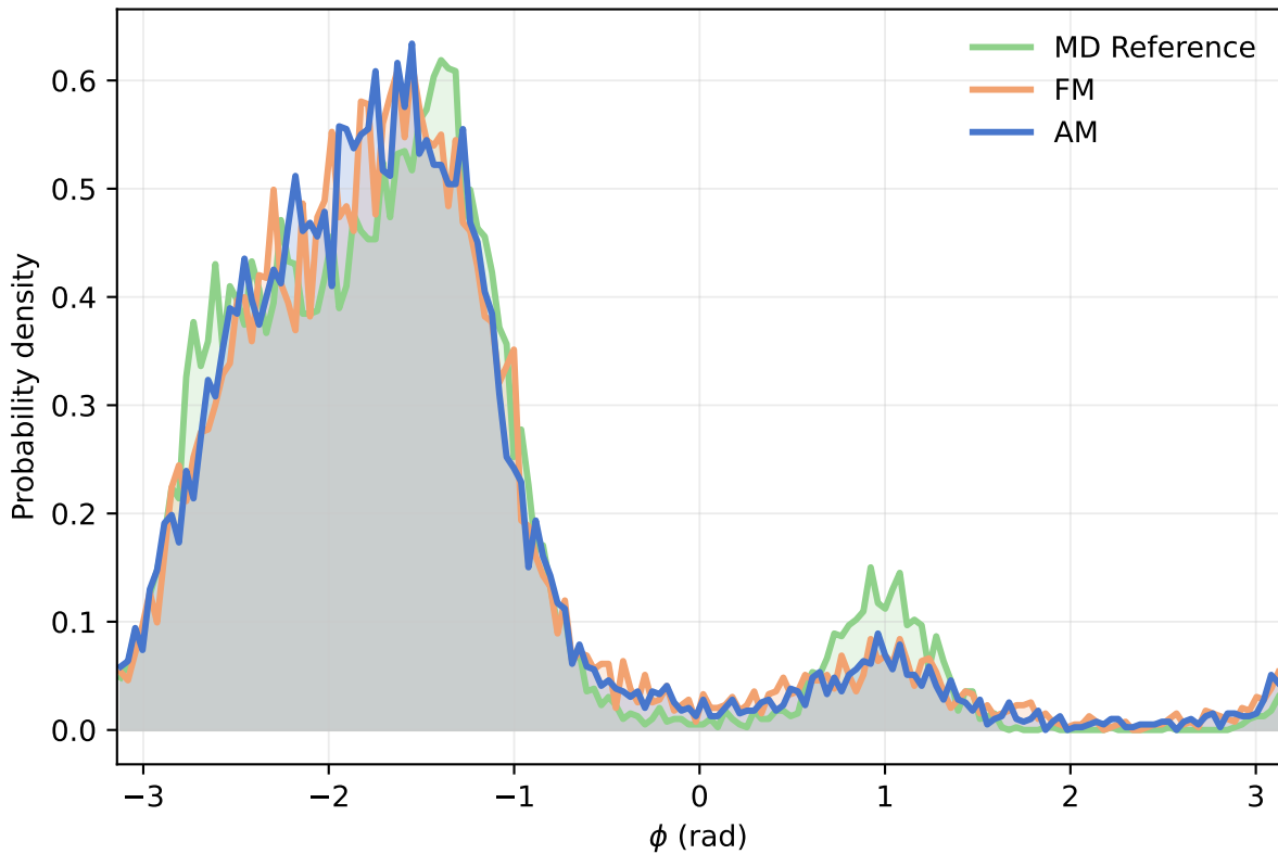
ADTM Ala2 800 K - phi marginal
