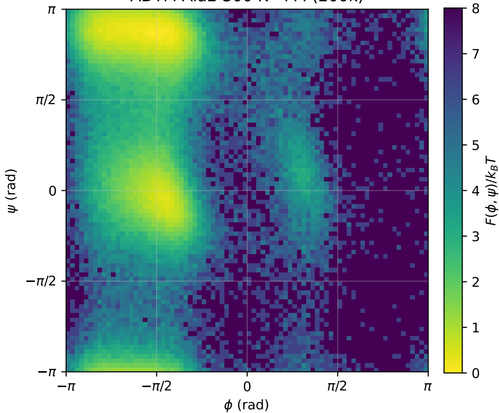
ADTM Ala2 300 K - FM (200k)
