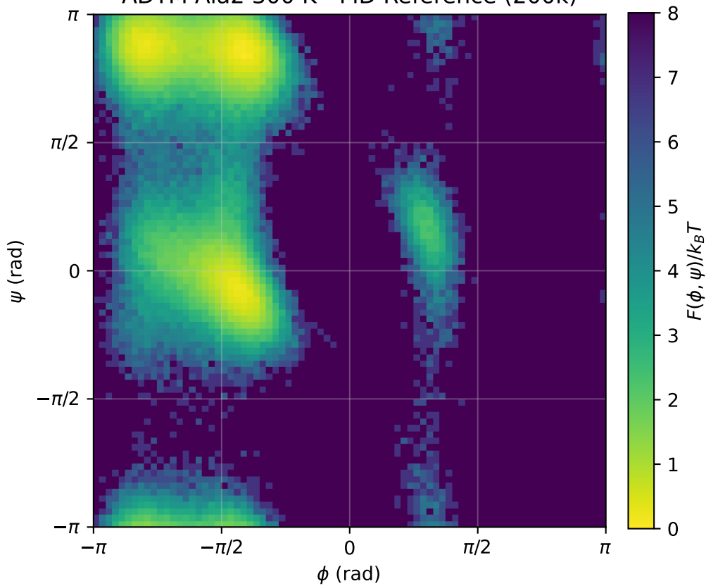
ADTM Ala2 300 K - MD Reference (200k)
