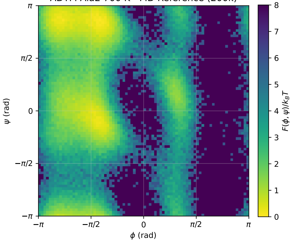
ADTM Ala2 700 K - MD Reference (200k)
