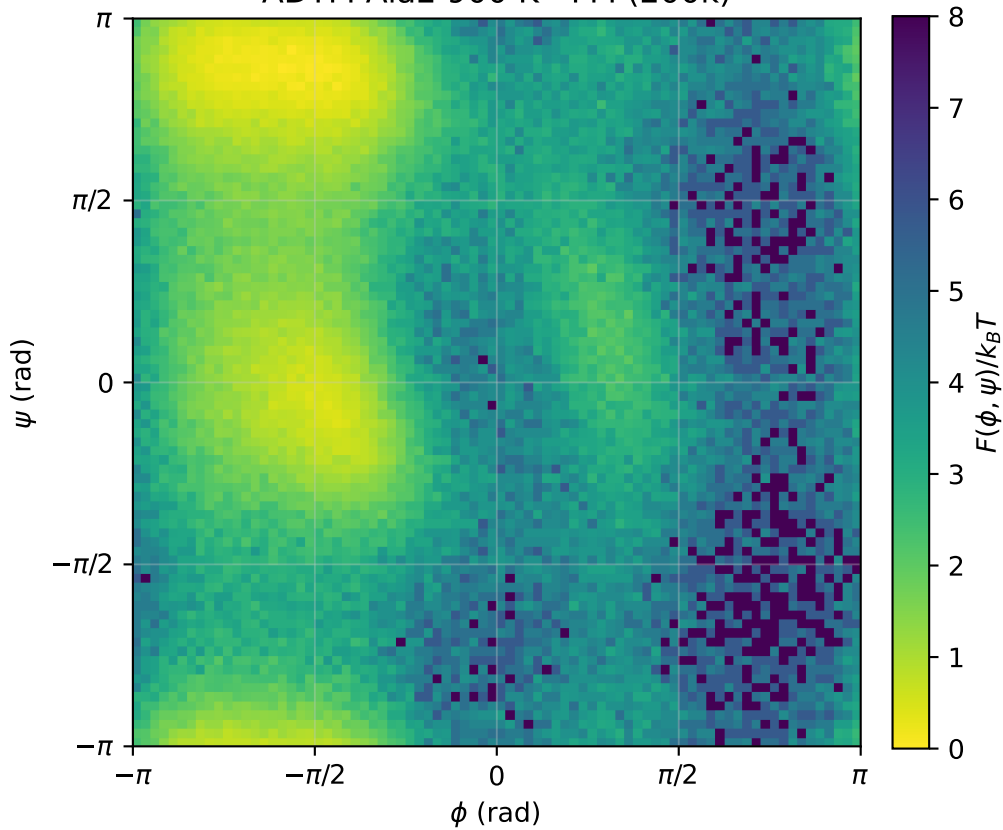
ADTM Ala2 900 K - FM (200k)
