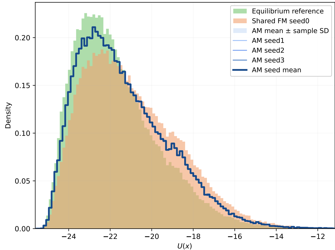
DW4 at \beta = 1.00 : energy distribution
