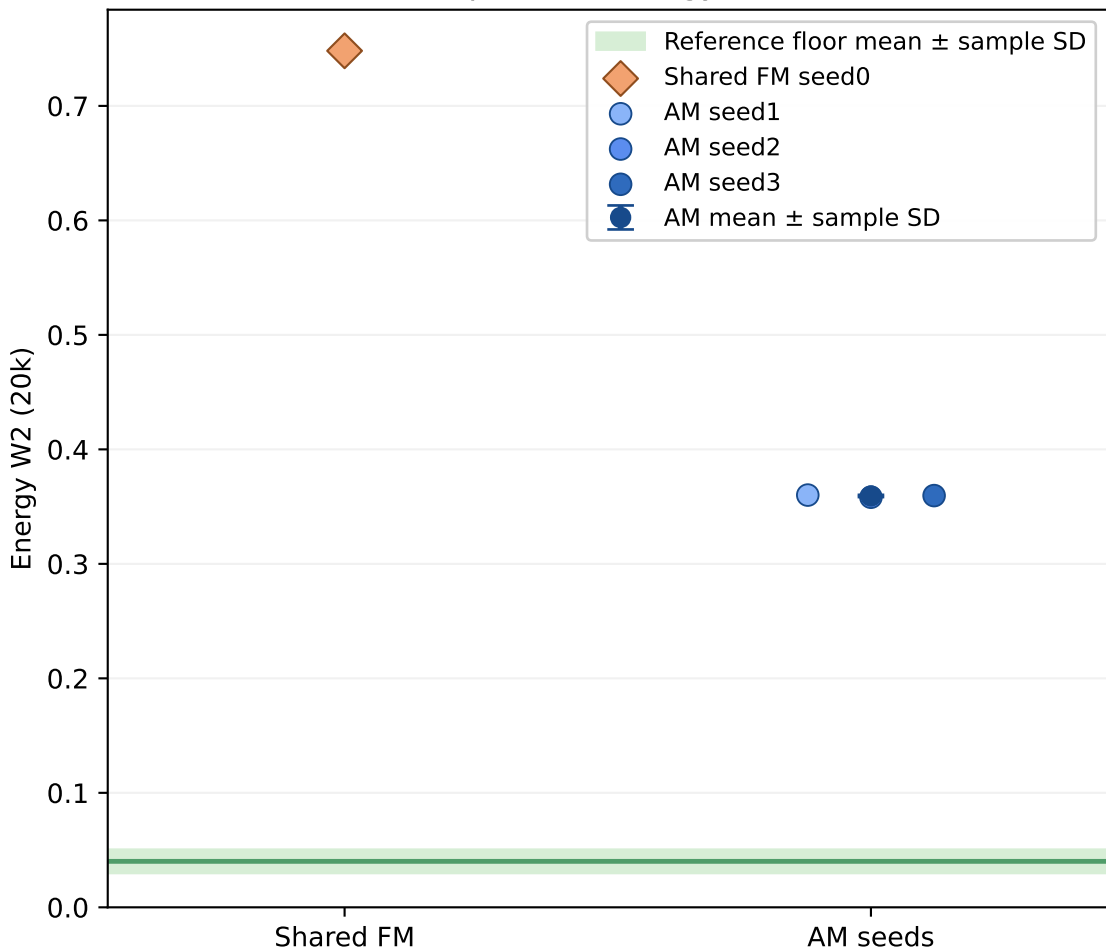
DW4 at \beta=1.00 : Energy W2 (20k)
