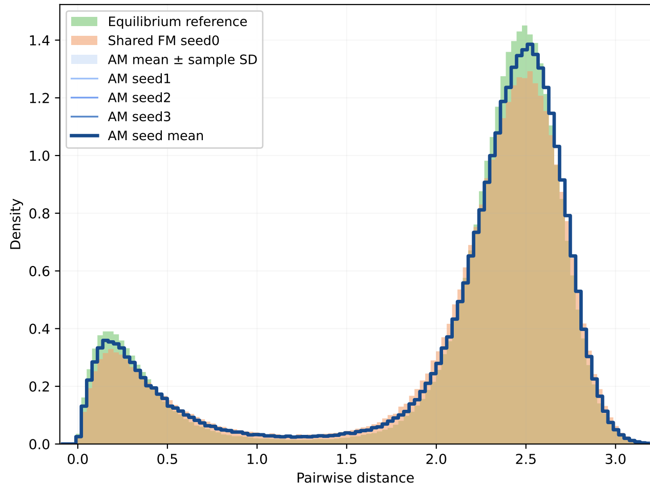
DW4 at \beta = 1.00 : pairwise distances
