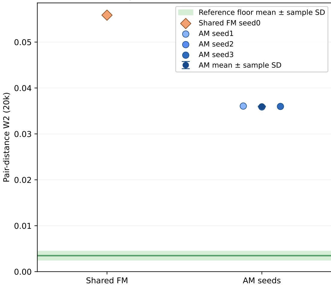
DW4 at \beta=1.00 : Pair-distance W2 (20k)
