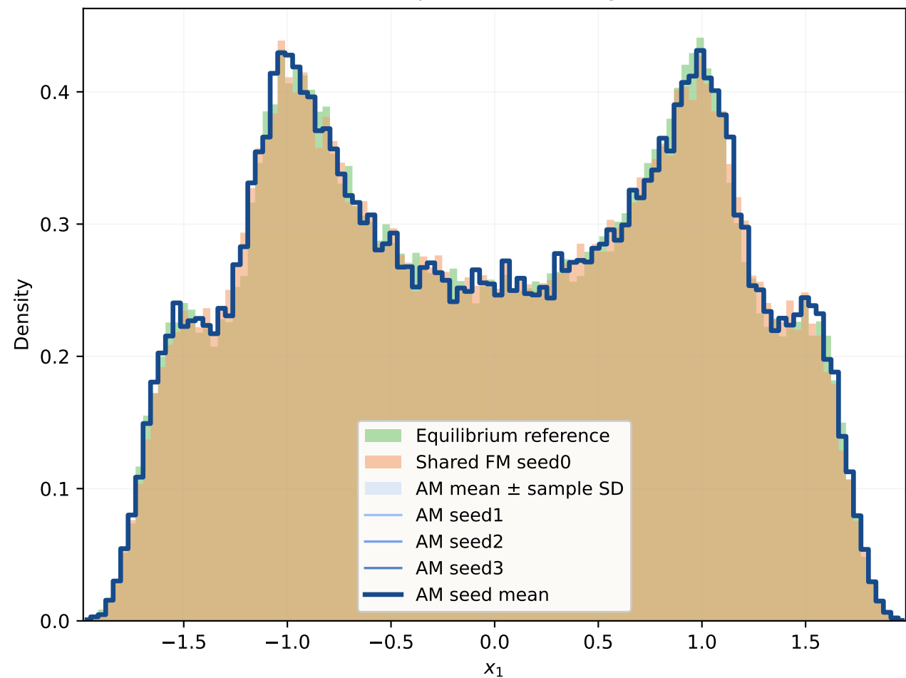
DW4 at \beta = 1.00 : x_1 marginal
