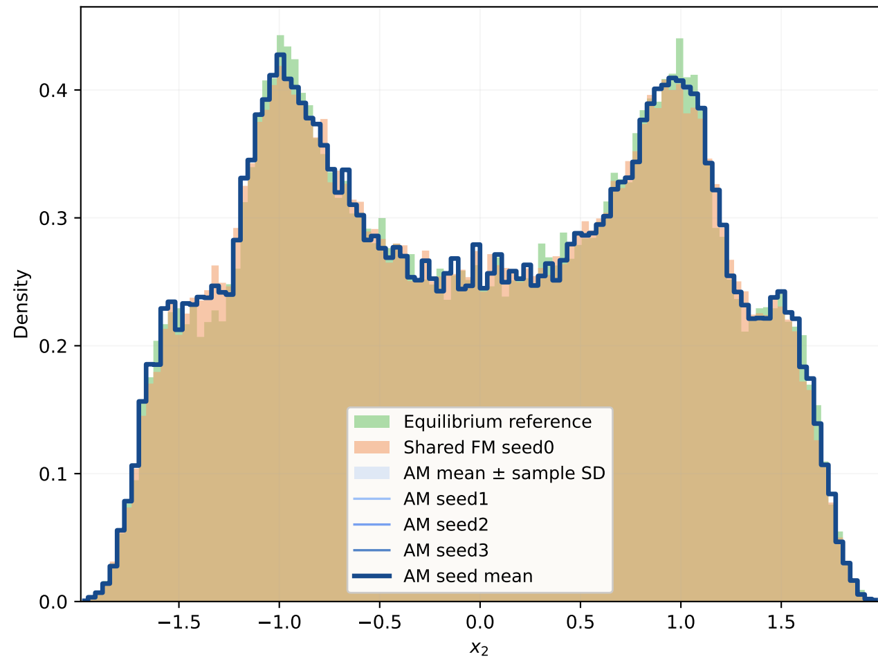
DW4 at \beta = 1.00 : x_2 marginal
