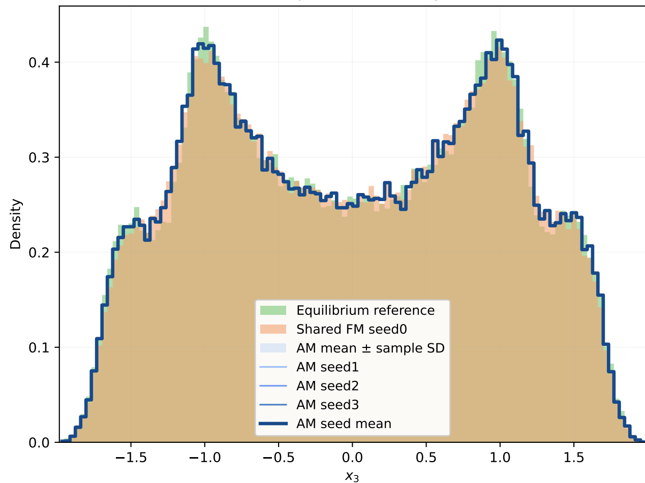
DW4 at \beta = 1.00 : x_3 marginal
