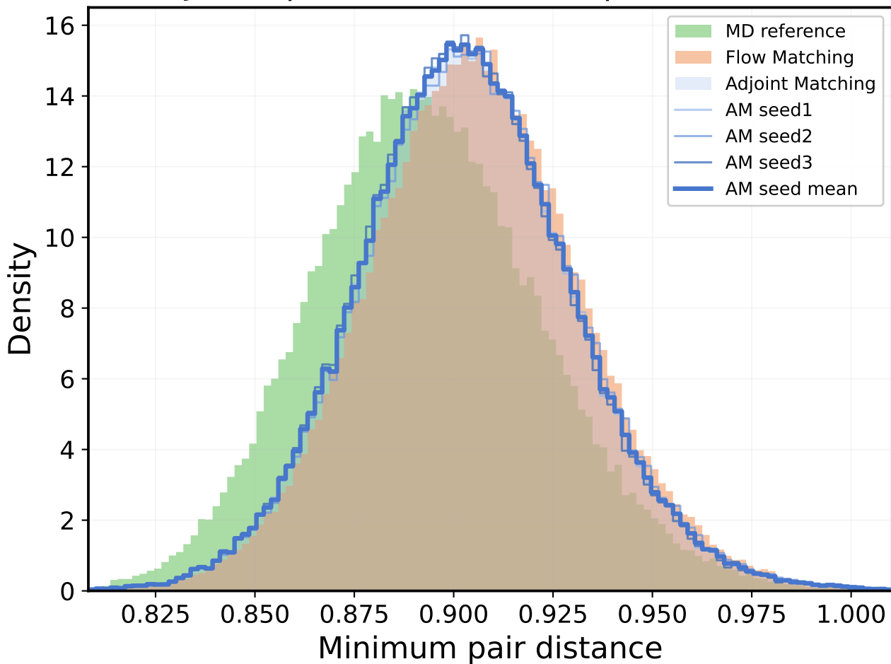
LJ13 at \beta = 1.00 : minimum pair distance
