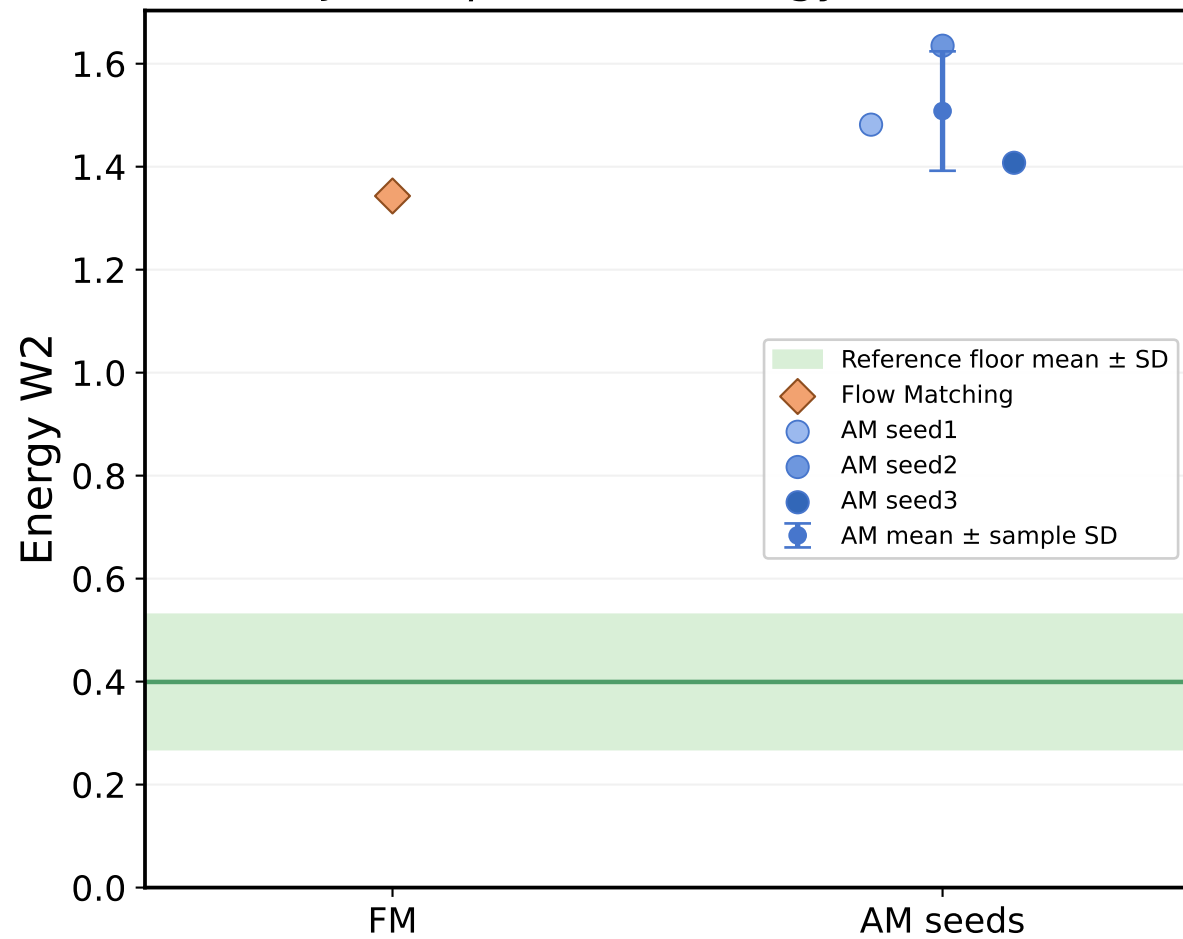
LJ13 at \beta = 1.00 : energy W2 (2k)
