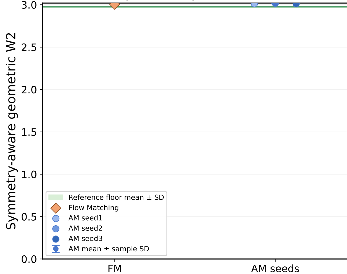
LJ13 at \beta = 1.00 : geometric W2 (2k)
