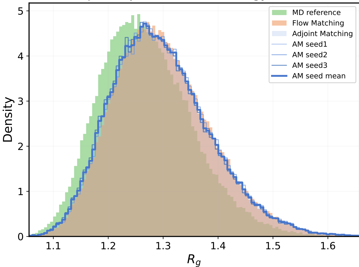
LJ13 at \beta = 1.00 : radius of gyration
