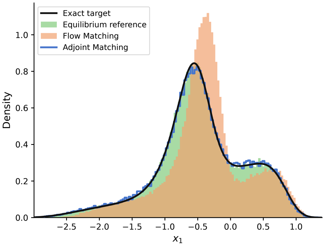
x_1 distribution, \beta = 1.20
