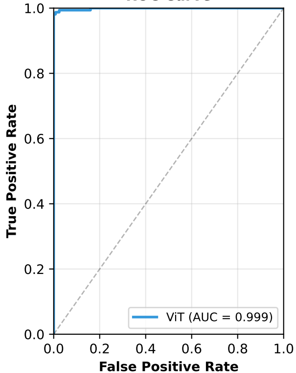
ViT Binary Classifier ROC Curve
