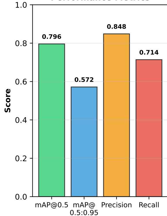
YOLO Object Detector Performance Metrics
