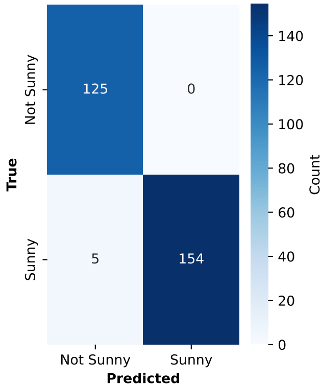
ViT Confusion Matrix Accuracy: 0.982
