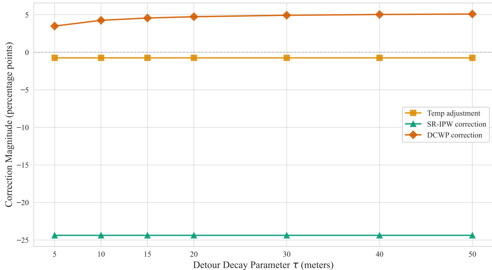
Magnitude of Each Bias Correction vs. \tau
