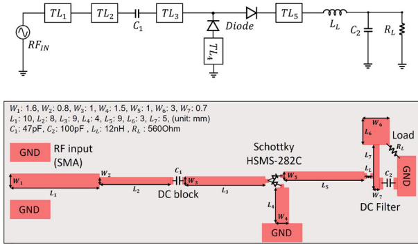
Fig. 6. Half-wave rectifier circuit: schematic (top) and layout (bottom).
