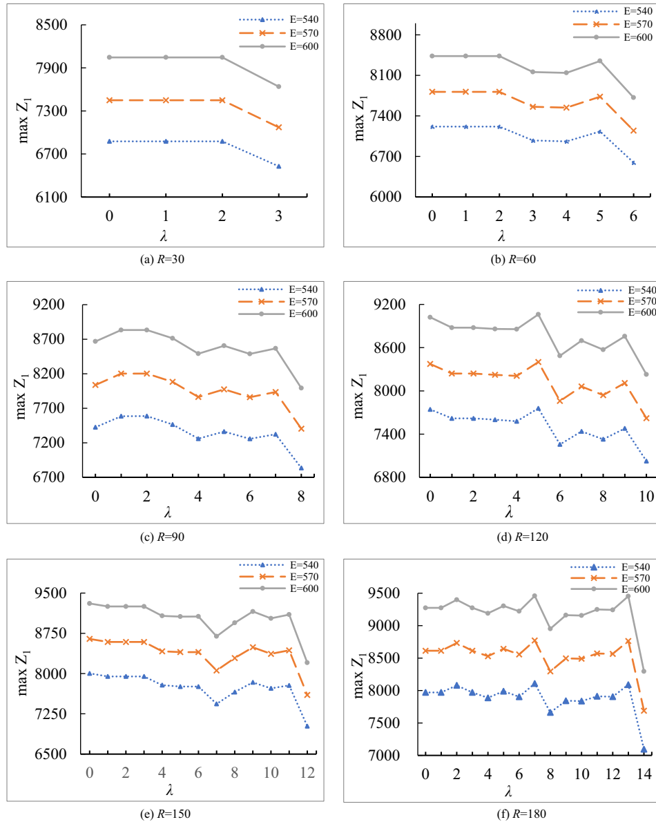
Fig. 5. Optimal evacuation traffic objective function values under different rescue traffic demands.
