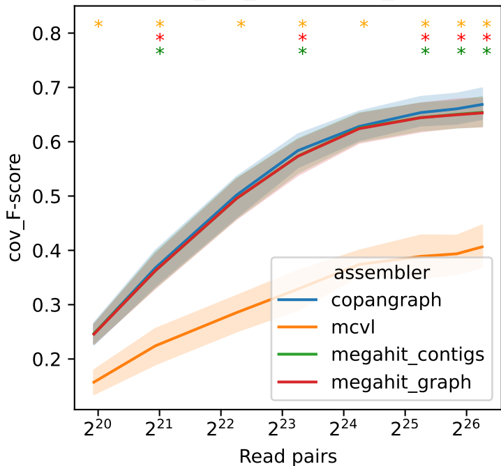
megahit_cov_F-score cov_F-score
