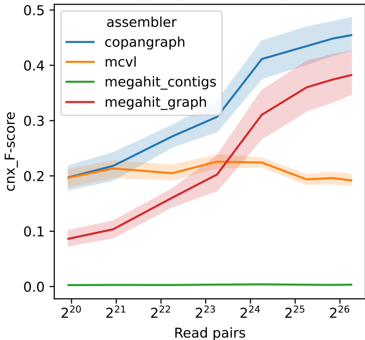
megahit_cnx_F-score cnx_F-score
