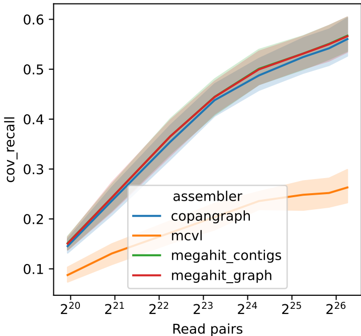
megahit_cov_recall cov_recall
