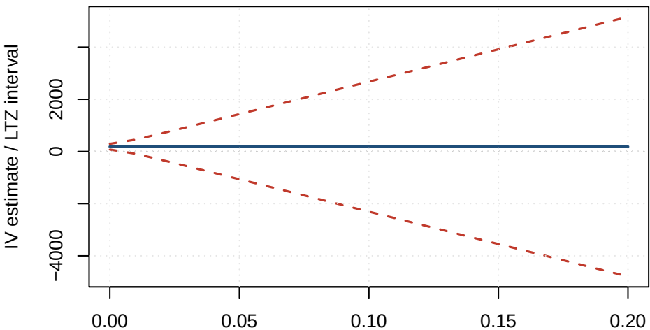
Maize: Uniform direct effect
