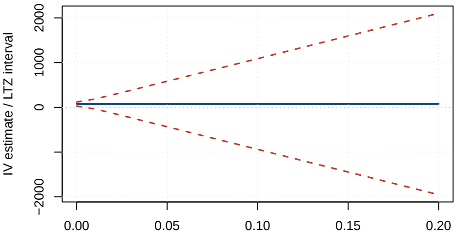
Wheat: Uniform direct effect
