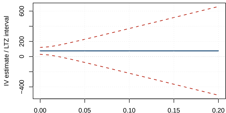
Wheat: Sparse/bare direct-effect pattern
