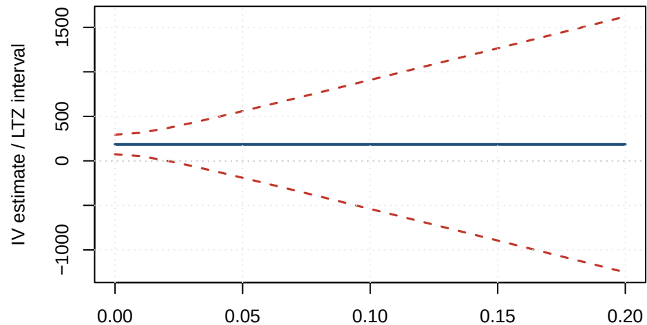
Maize: Sparse/bare direct-effect pattern
