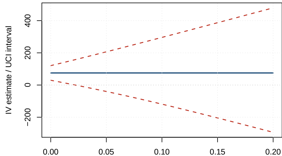
Wheat: Sparse/bare direct-effect pattern
