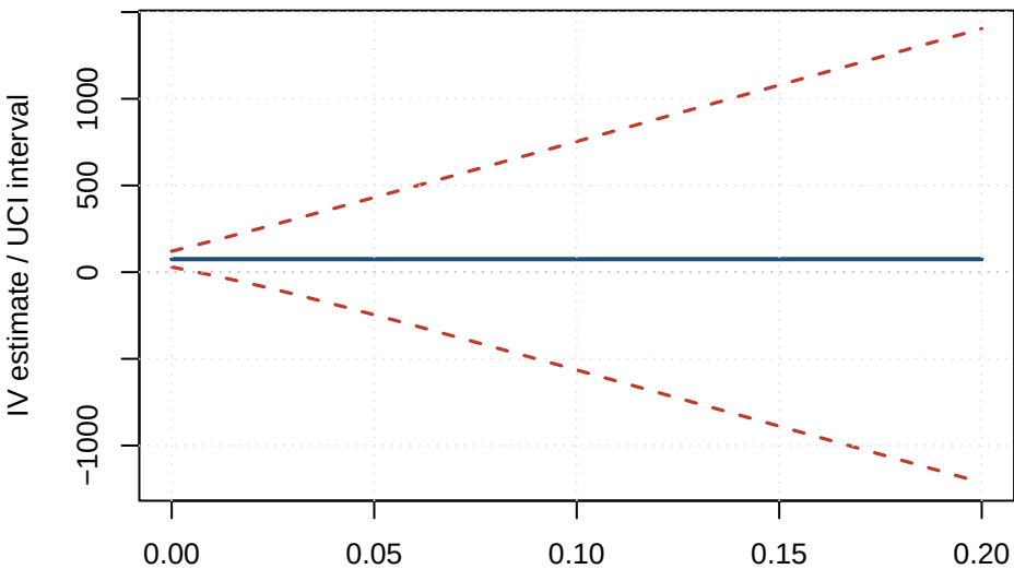
Wheat: Uniform direct effect
