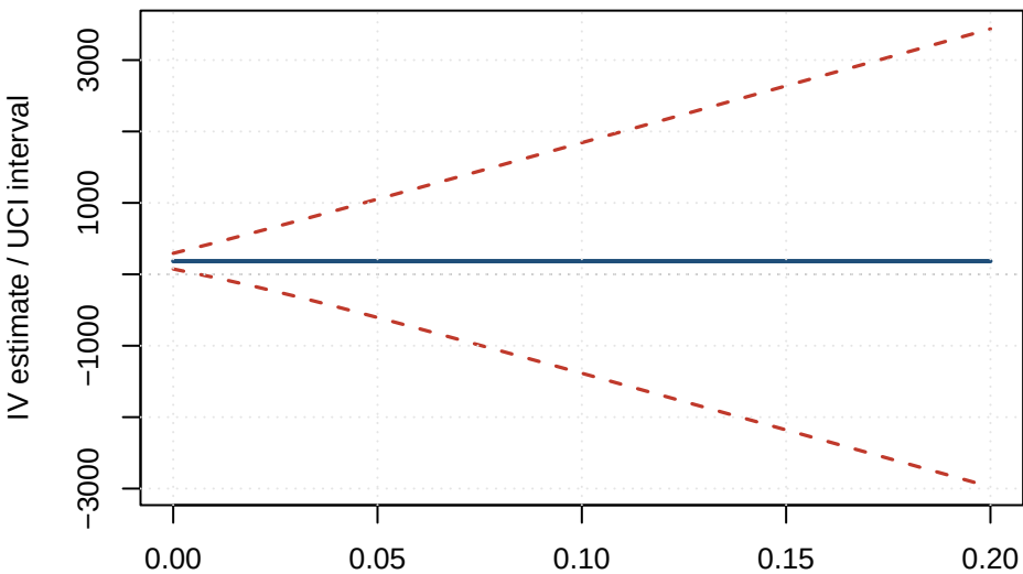
Maize: Uniform direct effect
