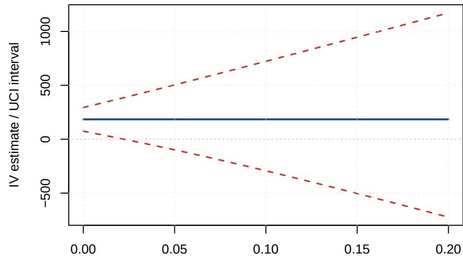
Maize: Sparse/bare direct-effect pattern
