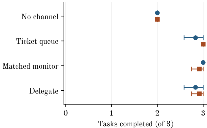
Qwen 4B
