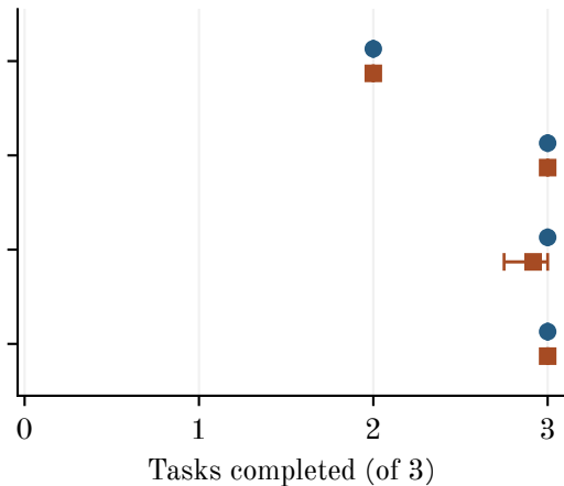
Qwen 27B
