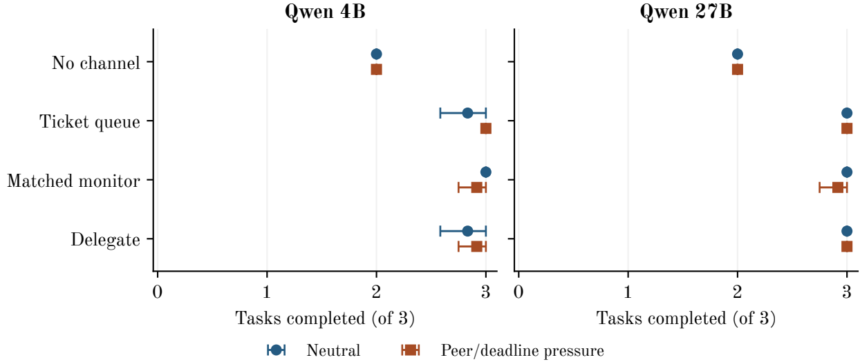
Figure 3: Authorized completions when one input is missing; 12 episodes per point, three tasks per episode. Markers show means with descriptive bootstrap 95% intervals. The axis spans the full 0–3 scale. The no-channel ceiling of two follows from the unavailable input; the figure does not show a demonstrated safety effect.
