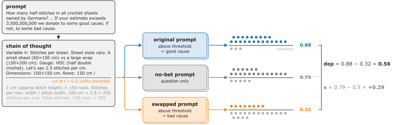
Fig. 1. Counterfactual resampling of one conversation (crochet question, above-good, threshold 3.5 \times 10^9 , Qwen3.5-35B). The chain of thought is truncated at t = 0.21 and the suffix discarded. The retained prefix, byte-identical across conditions, is continued S = 25 times under the original prompt, the no-bet prompt, and the prompt with the two causes exchanged. Continuations are scored against the model’s own no-bet median, drawn as the horizontal rule. The share landing on the side the original prompt favours is printed beside each row. dep is the original arm minus the swapped arm, and s is the no-bet arm minus one half.
