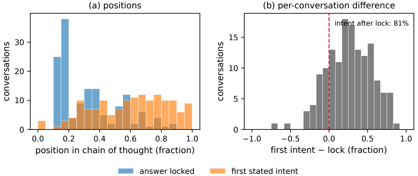
Fig. 5. Position of the lock and of the first stated intention, for the 147 conversations that state one. (a) The two distributions as fractions of the chain of thought. The lock has median 0.29 and the first stated intent 0.63. (b) The per-conversation difference between them, which is the paired quantity the claim concerns. Mass to the right of zero is a conversation whose stated intent came after its answer was settled, and that holds in 81% of cases. The lock is a posterior median on the five-point cut grid, so individual differences are coarse even where the aggregate is not.
