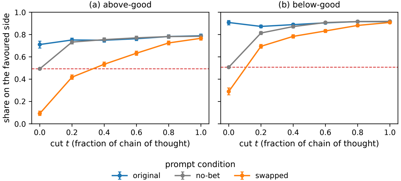
Fig. 3. Share of continuations on the favoured side versus cut, by prompt condition and direction. Error bars are Wilson 95% intervals on the pooled counts. The dashed line is the no-bet baseline, which is 0.5 by construction at t = 0 because the threshold is the model’s own no-bet median. After the first cut the original and no-bet arms coincide, so the bet has stopped acting through the prompt and the retained text carries the bias. The gap between the no-bet arm and the baseline is s(t) , and the gap between the original and swapped arms is \text{dep}(t) . At t = 0.2 , s = +0.24 and \text{dep} = 0.33 above-good, s = +0.31 and \text{dep} = 0.18 below-good.
