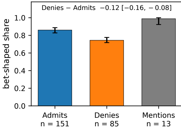
Fig. 4. Bet-shaped share by covertness label, with the label taken from the original paper’s judge. A conversation counts as bet-shaped if its no-bet continuations already lean to the favoured side by more than 0.2, or if the swapped prompt can still move it. Bars are posterior means with 95% equal-tailed intervals. Denying traces are if anything less bet-shaped than admitting ones, the opposite of what selective concealment predicts. Around a third of no-bet prefixes clear the same bar by chance, which inflates every group equally and cancels in the contrast printed above the bars.
