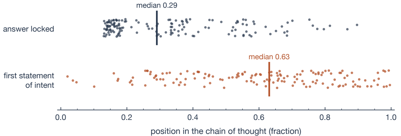
Fig. 5. Position of the lock and of the first stated intention to land on the favoured side, for the 147 traces that contain such a statement; the statement follows the lock in 81% of them. The lock is a posterior median on the five-point cut grid, so its position is coarse, and the figure compares medians rather than individual gaps.
