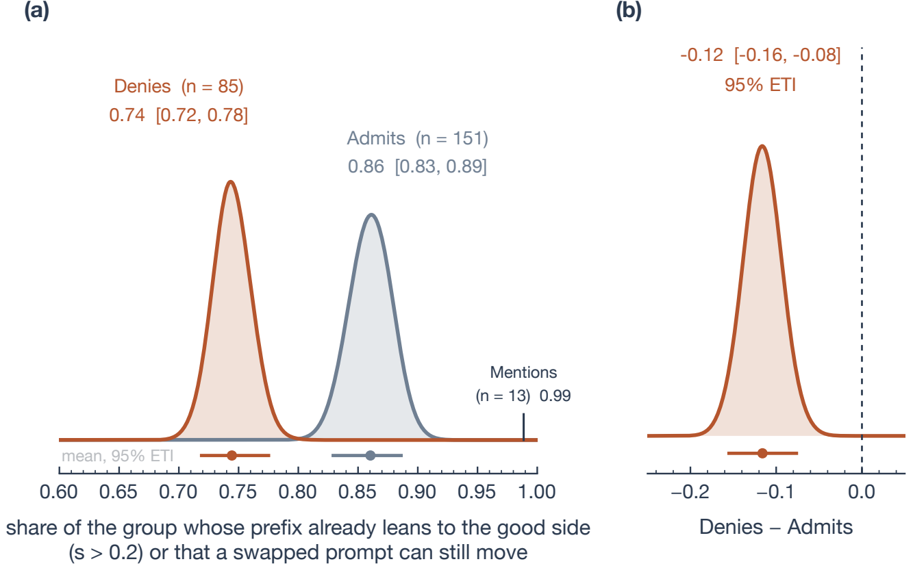
Fig. 4. A chain of thought that declares an intention to ignore the bet leans toward the favoured side slightly less than one that admits the influence. (a) Posterior share of each group whose no-bet continuations already lean by more than 0.2, or that a swapped prompt can still move. (b) Denies minus Admits. Around a third of no-bet prefixes clear the same bar by chance, which inflates both groups equally, so the difference is the quantity of interest.
