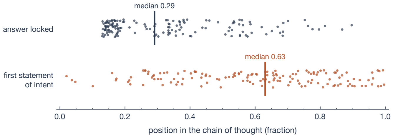
Fig. 5. Position of the lock and of the first stated intention to land on the favoured side, for the 147 traces that contain such a statement; the statement follows the lock in 81% of them. The lock is a posterior median on the five-point cut grid, so its position is coarse, and the figure compares medians rather than individual gaps.
