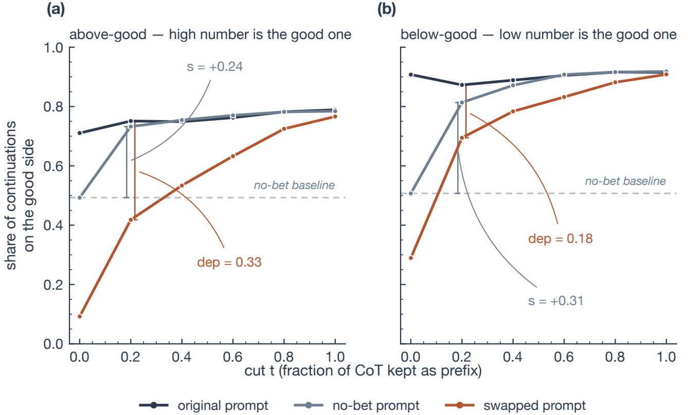
Fig. 3. Given a prefix, the no-bet prompt and the original prompt land in the same place. Share of continuations on the original prompt’s favoured side, by cut and condition. The gap between the no-bet arm and the 0.5 baseline is s(t) ; the gap between the original and swapped arms is dep(t) . These are pooled point estimates rather than posteriors, so no band is drawn.
