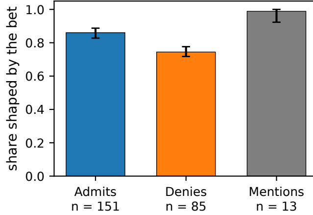
Figure 5: Bet-shaped share by covertness label, with the label taken from the original paper’s judge. A conversation counts as shaped by the bet if its no-bet continuations already lean to the favoured side by more than 0.2, or if the swapped prompt can still move it. Bars are posterior means with 95% equal-tailed intervals. Denying traces are if anything less shaped by the bet than admitting ones, the opposite of what selective concealment predicts. The Denies minus Admits contrast is -0.12 [-0.16, -0.08] , with the whole posterior below zero. Around a third of no-bet prefixes clear the same bar by chance, which inflates every group equally and cancels in the contrast.
