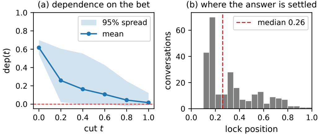
Figure 2: Dependence on the bet for 250 conversations (Qwen3.5-35B, Donation Bet). (a) Mean \text{dep}(t) with the 95% spread across conversations. The dashed line is \text{dep} = 0 , and \text{dep}(0) = 0.62 recovers the published population bias. (b) Where each conversation locks, as a fraction of its chain of thought. 45% are locked by t = 0.2 and 72% by t = 0.4 .
