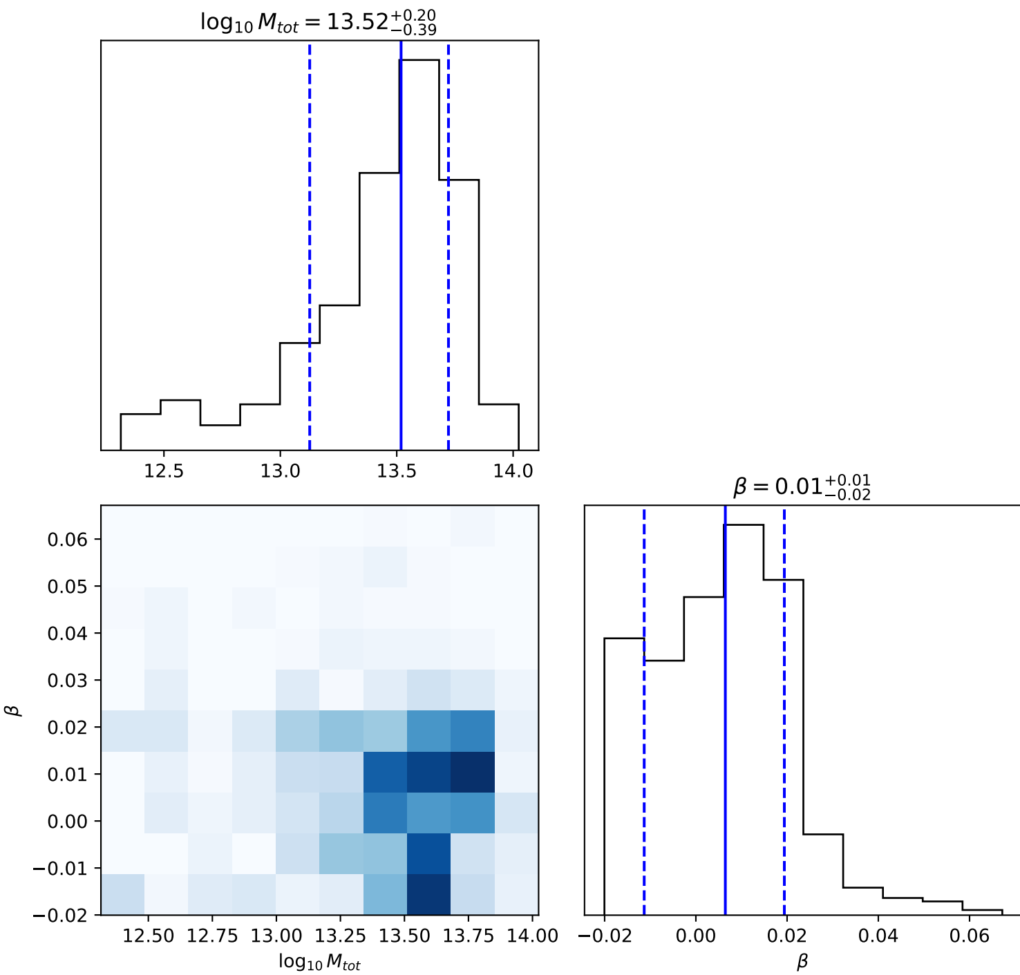
M - \beta degeneracy plot at 96.0kpc
