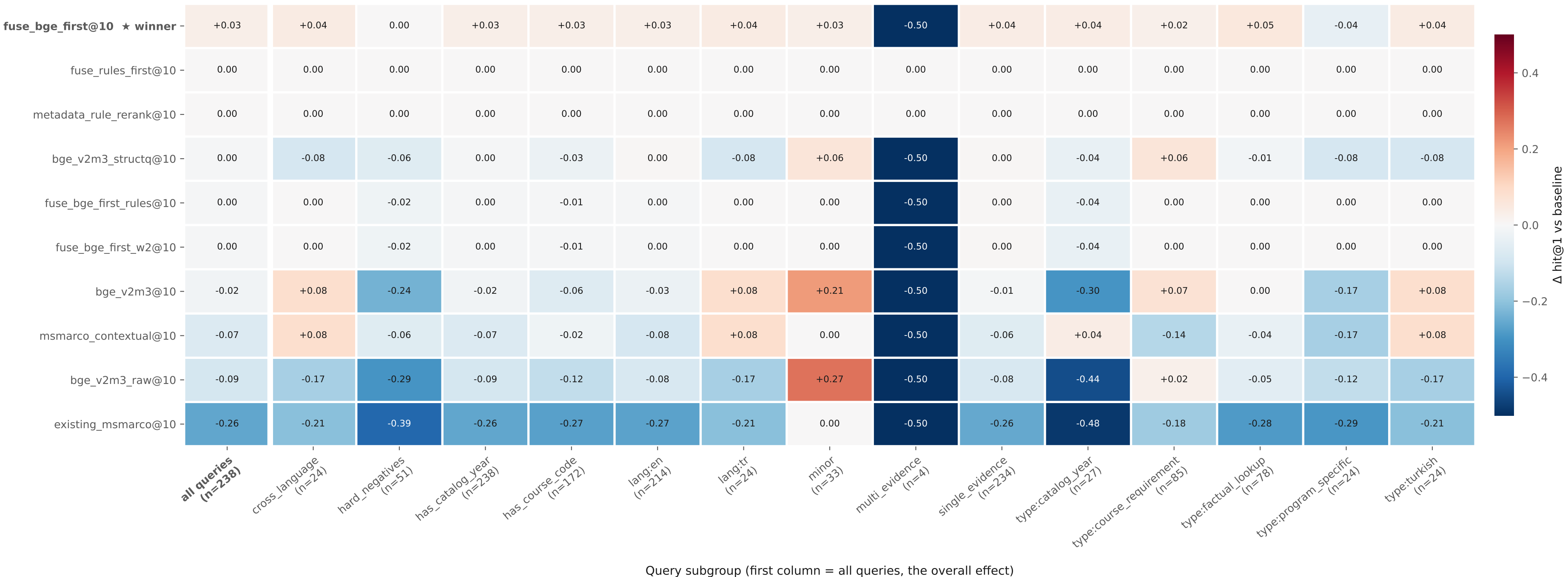
Where reranking helps and where it hurts (hit@1 vs 'original_ranking@10')
