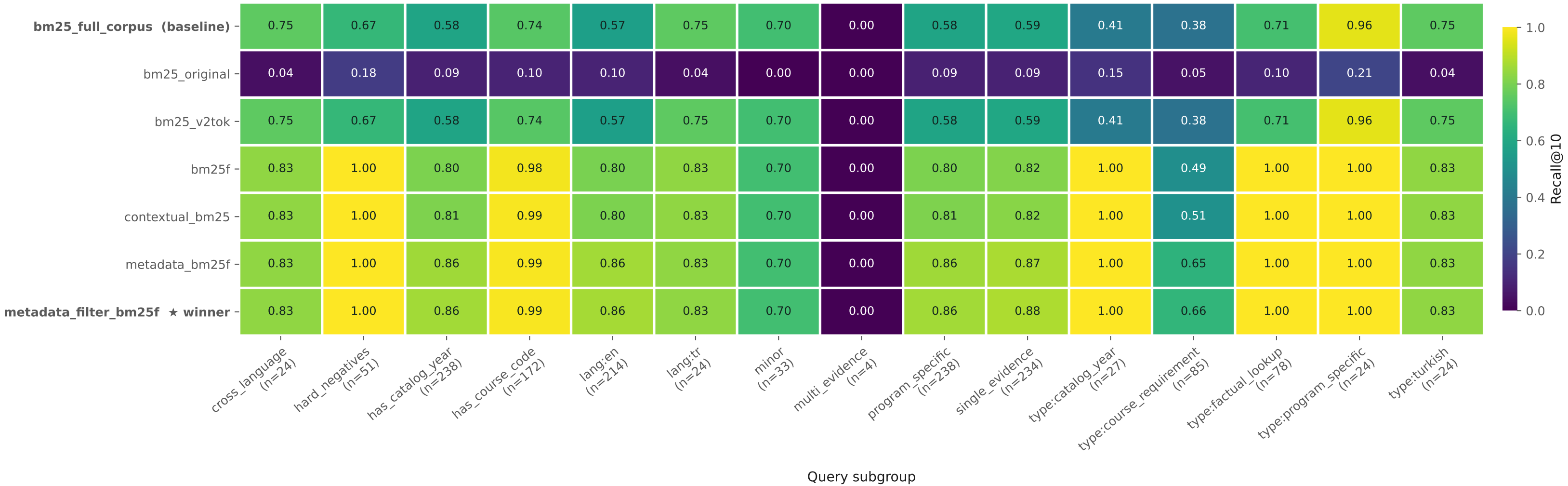
Recall@10 by method and query subgroup
