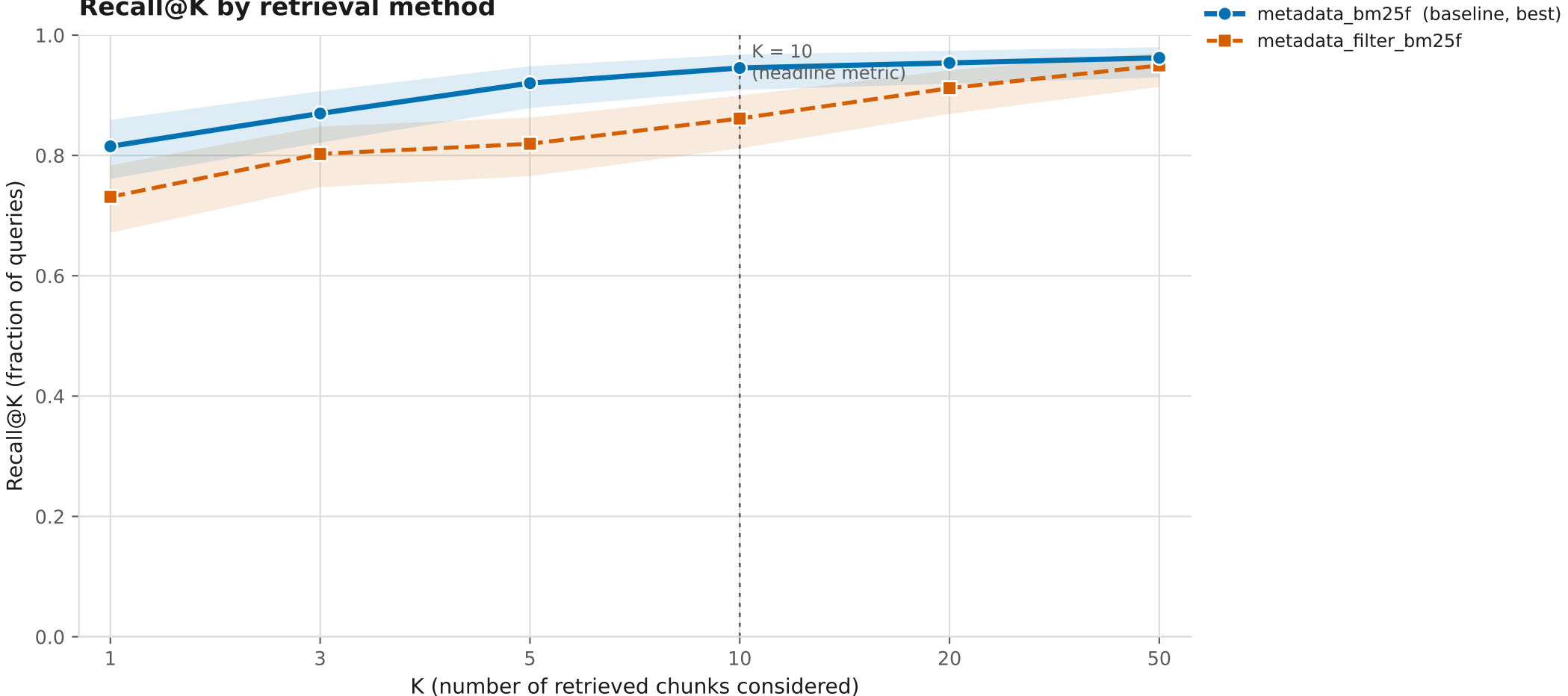
Recall@K by retrieval method
