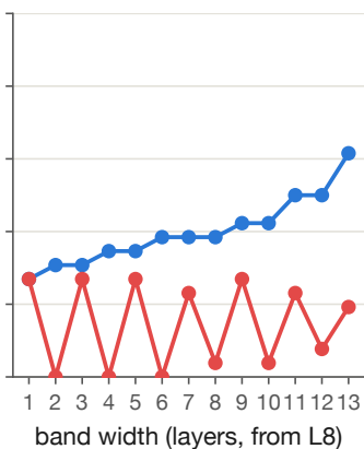
Qwen3.5-4B, n = 52
