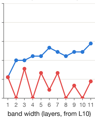
Qwen3-4B (dense attention), n = 45
