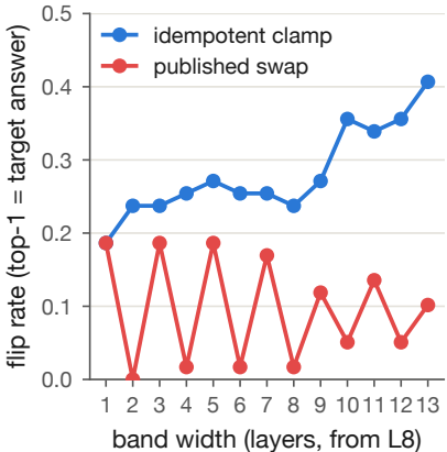
Qwen3.5-9B, n = 59
