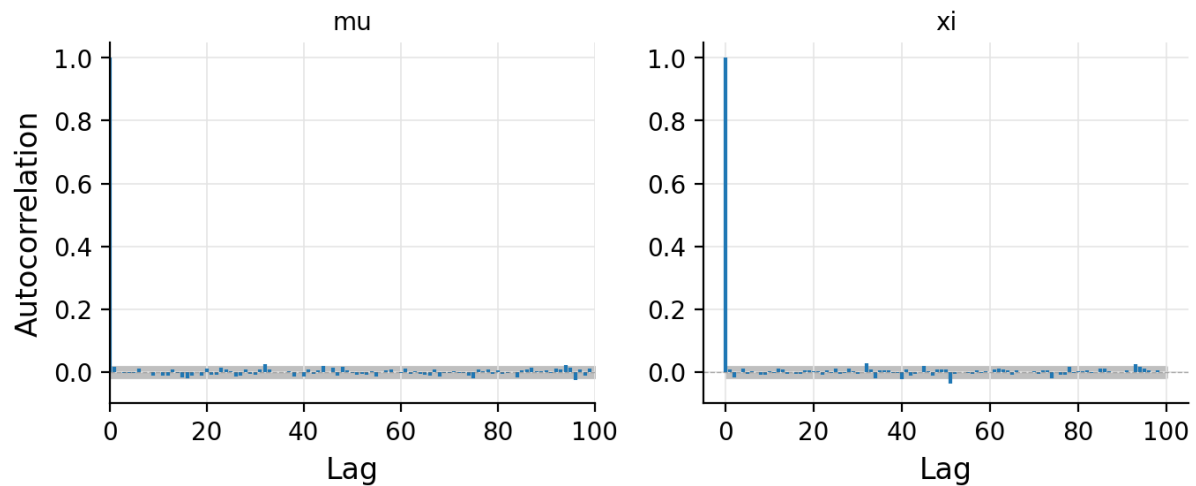
Figure 3 - Autocorrelation by lag for each parameter.
