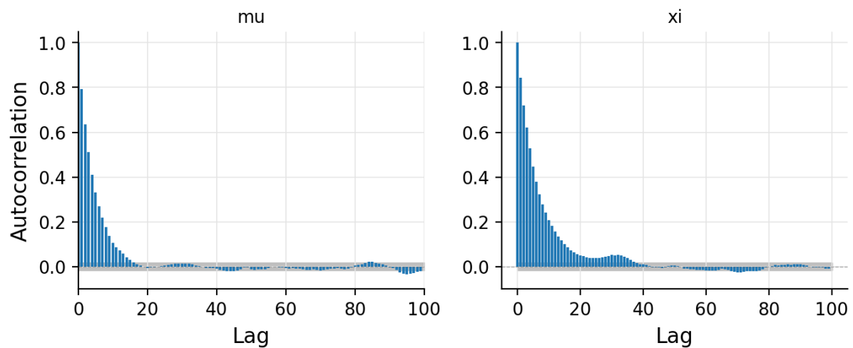
Figure 3 - Autocorrelation by lag for each parameter.
