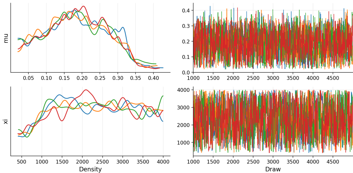
Figure 2 - Trace plots. Left: marginal posteriors; right: sample traces per walker.
