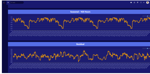
Fig. 18: 168-hour seasonality additionally residual component indicating unexpected performance losses in equipment operation.
