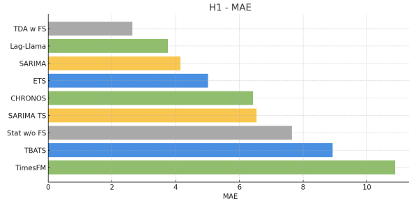
(a) MAE for H1 Dataset
