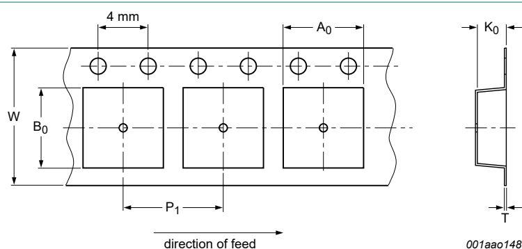
Fig. 3. Plastic/Embossed carrier tape
