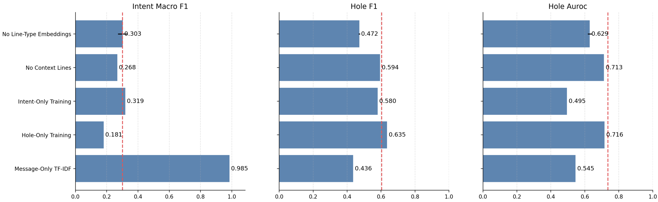
Ablation Results on the Full Experiment
