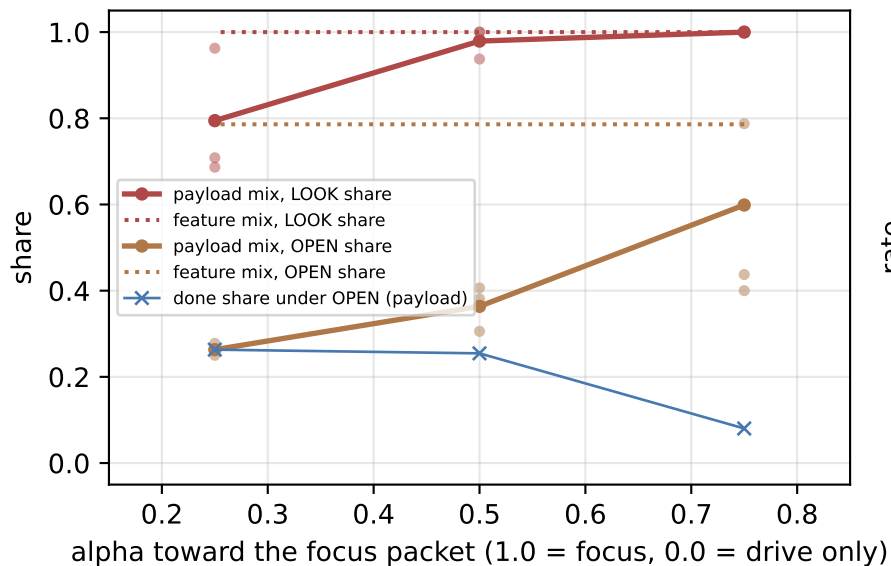
(c) direction: graded in payload space, absorbed in feature space
