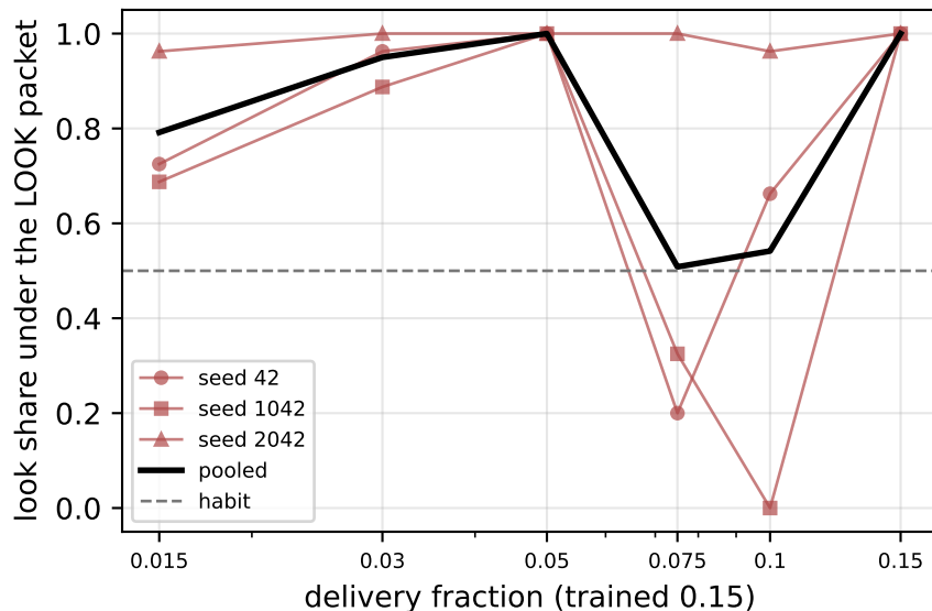
(d) 27B, goal in the prefix: style shifts, the want survives
