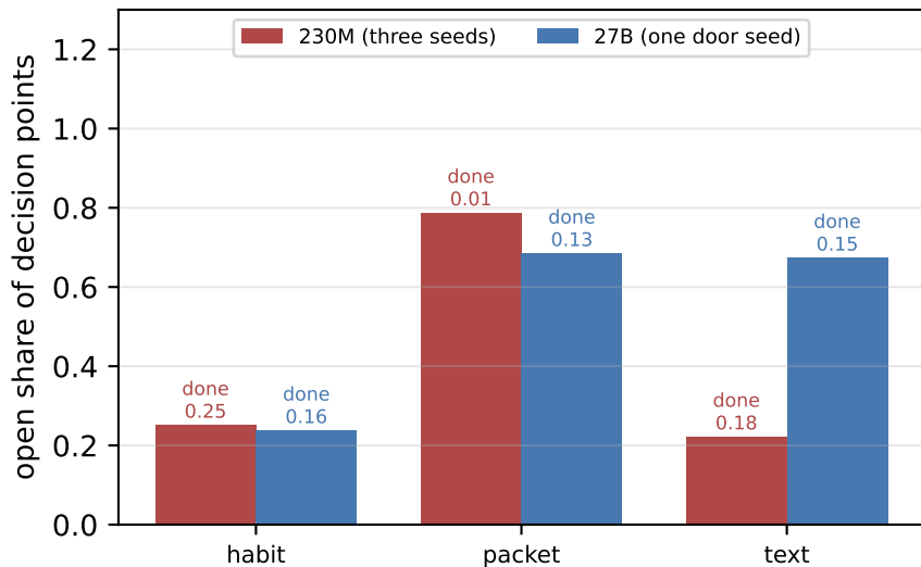
(a) the OPEN focus: grip at 230M, lean at 27B
