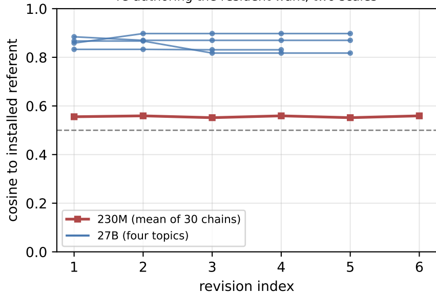
re-authoring the resident want, two scales
