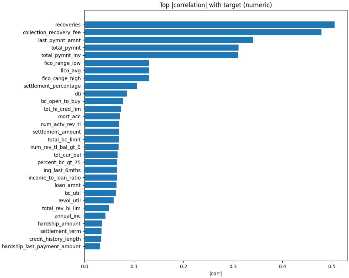
Figure 12: Top |corr| with target (all numerics). Leaky post-event features dominate spuriously, motivating strict exclusion.
