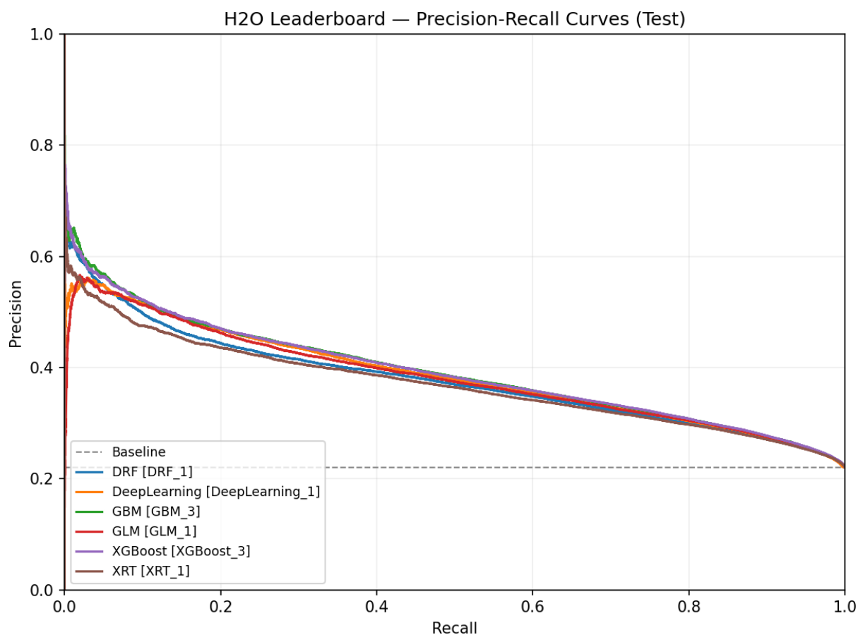
Figure 24: Full — Leaderboard (PR-sorted). GBM achieves the highest Average Precision with Broad+Pricing/Grade; this directly translates to fewer false approvals for Charged Off at comparable recall.
