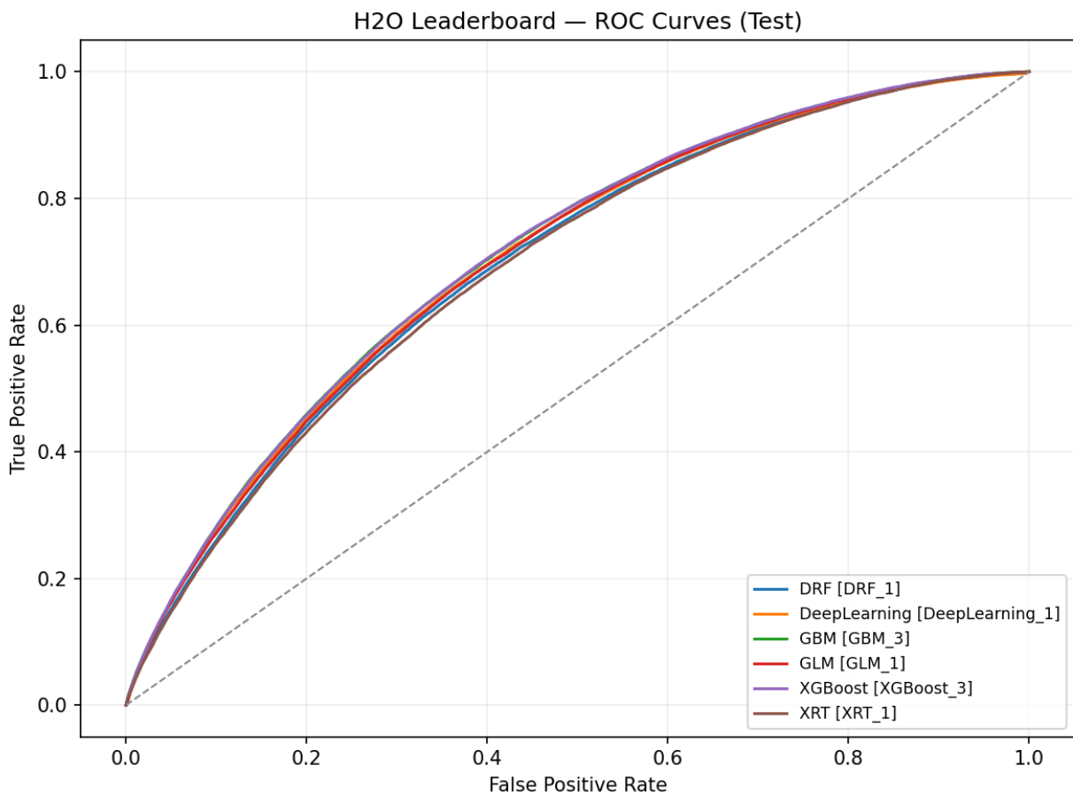
Figure 25: Full — Leaderboard (ROC-sorted). Tree ensembles dominate ROC; consistent ranking enables reliable threshold selection for Charged Off detection on out-of-time data.
