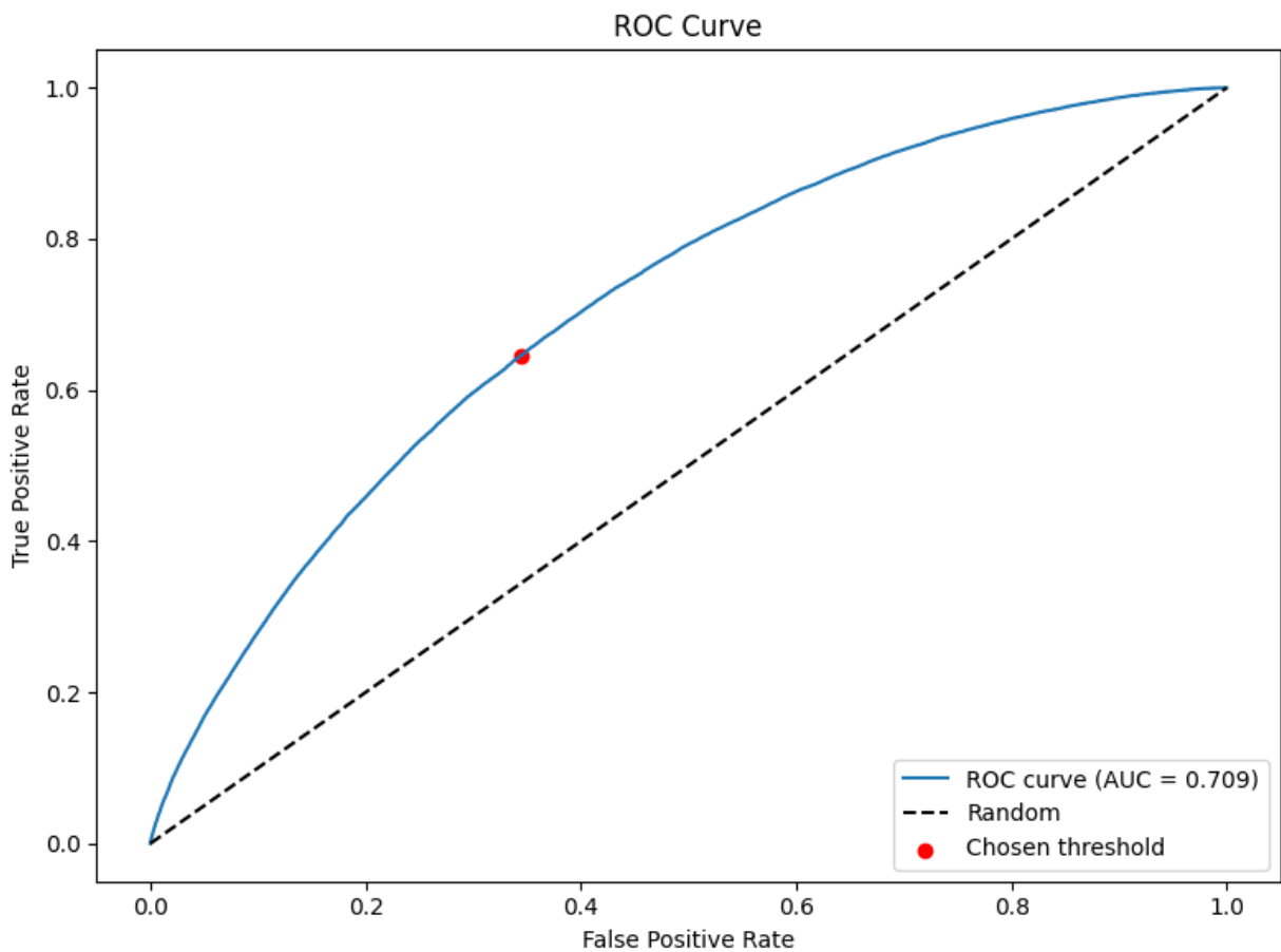
Figure 23: Full — ROC curve (winner). Winner: GBM. ROC complements PR by confirming ranking stability at production scale, important when prevalence and drift vary.
