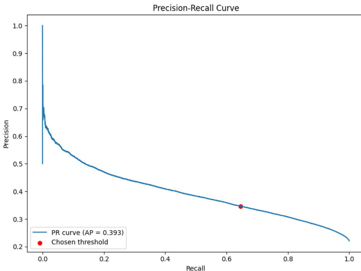
Figure 22: Full — Precision–Recall curve (winner).
