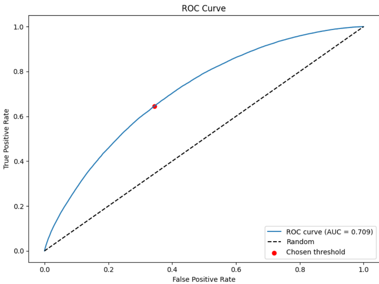
Figure 23: Full — ROC curve (winner).
