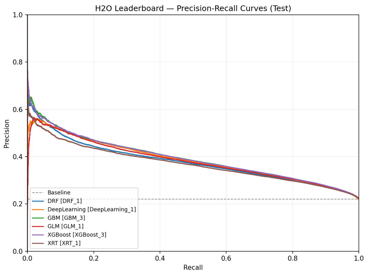
Figure 24: Full — Leaderboard (PR-sorted).
