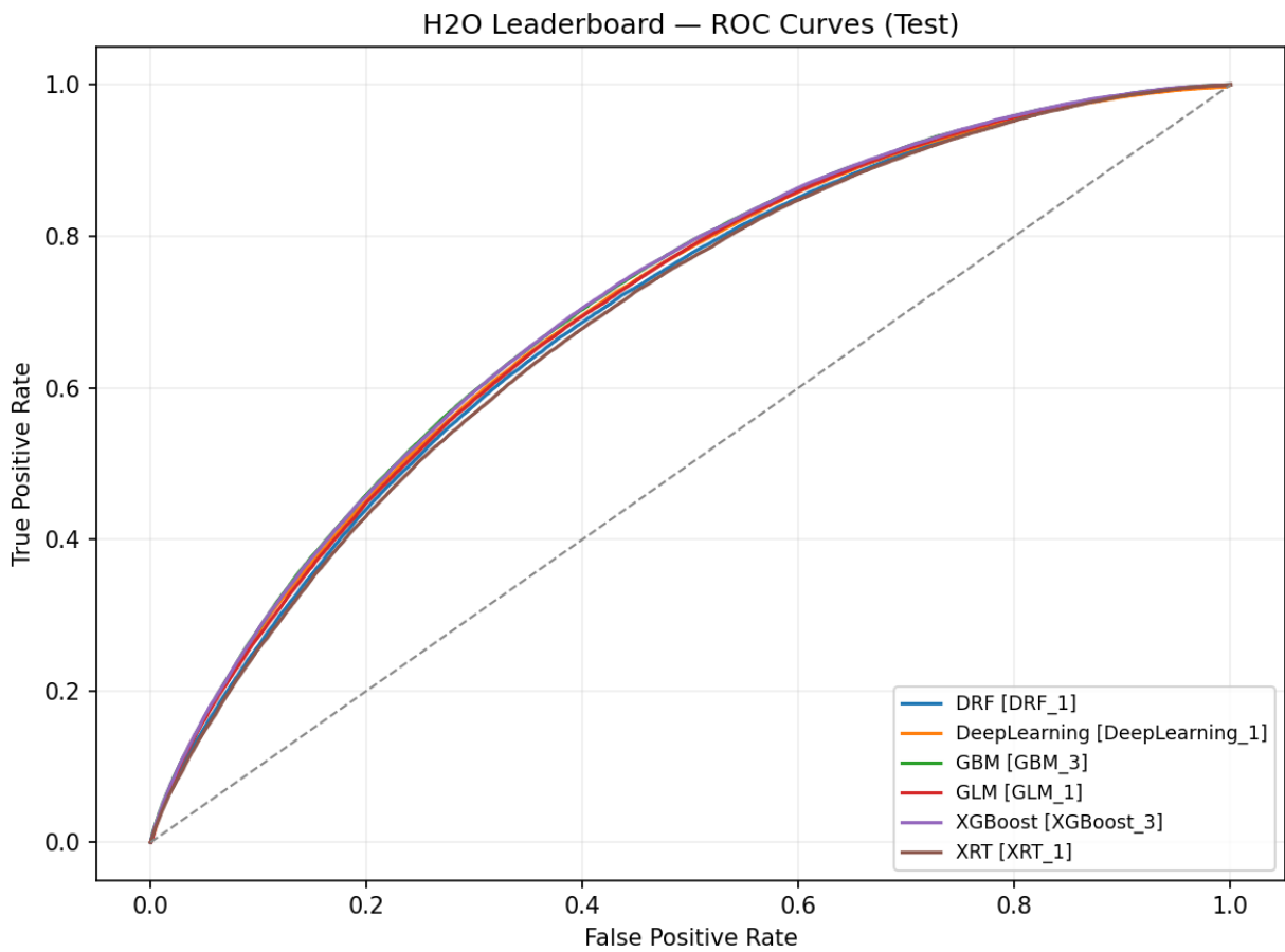
Figure 25: Full — Leaderboard (ROC-sorted).
