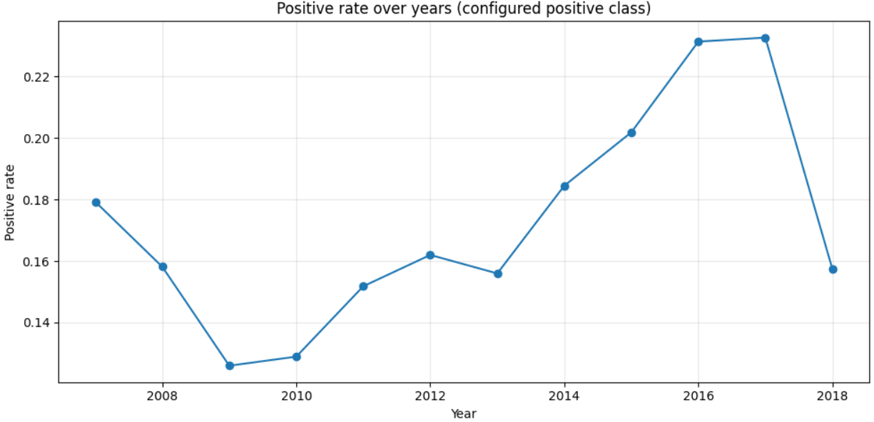
Figure 1: Positive rate by year (class balance). Highlights rising defaults into 2016–2017, then a dip in 2018 due to right-censoring/volume changes.
