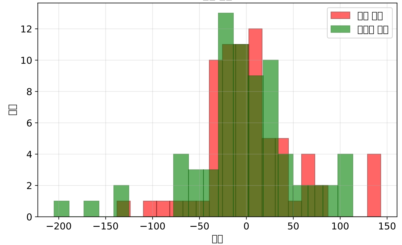
Model coefficients
