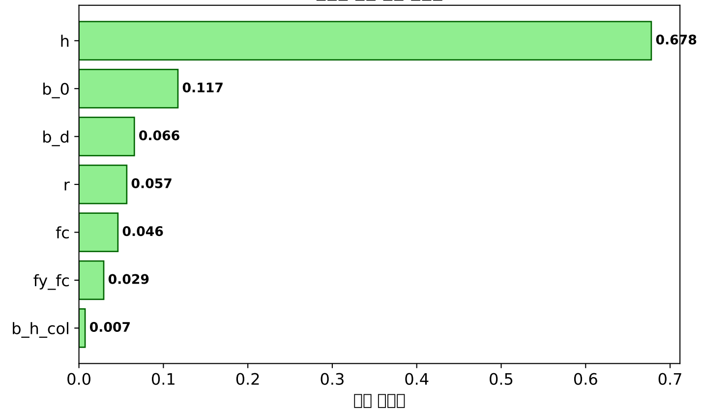
Model coefficients
