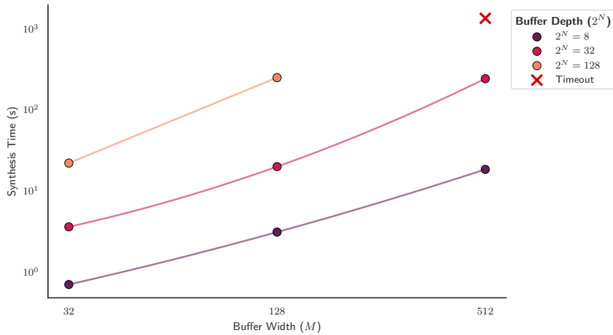
Figure 6.2: Synthesis time (log scale) versus entry width for each buffer depth. The red cross at N = 7 , M = 512 marks a timeout.
