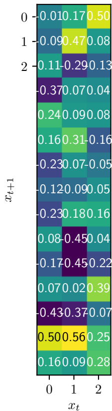
A — Mode Projection.
