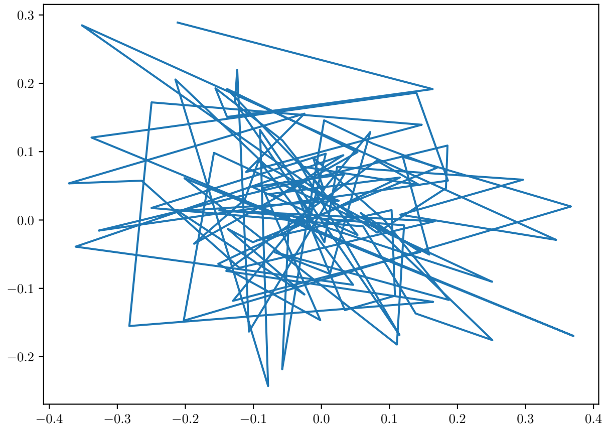
y_t — Observable Sequence 3
