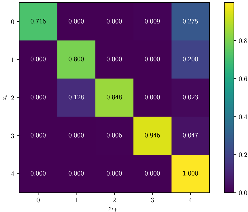
\pi[z_t, z_{t+1}] — Transition Probs.
