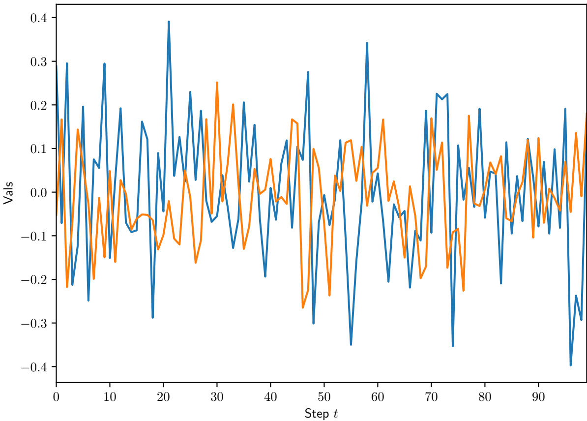
y_t — Observable Sequence 1
