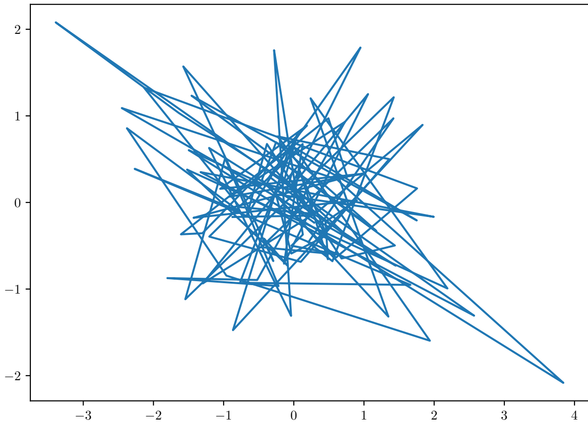
y_t — Observable Sequence 1
