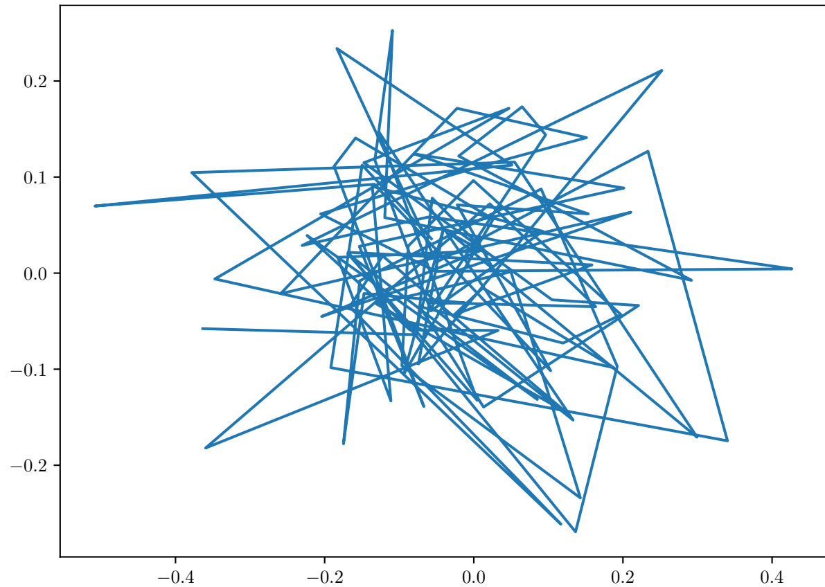
y_t — Observable Sequence 4
