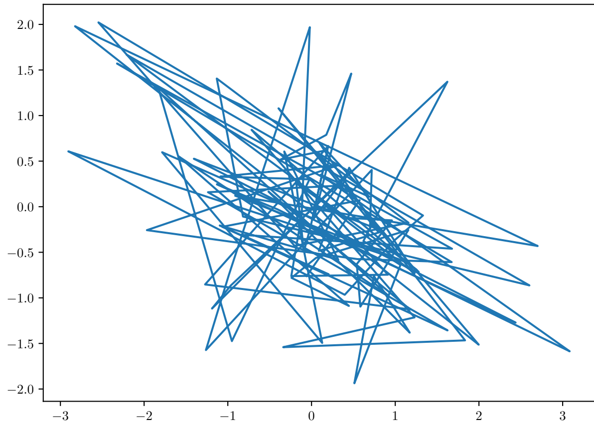
y_t — Observable Sequence 2
