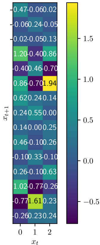
\Sigma — Mode Covariance.
