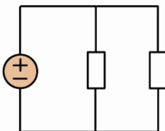
Figur 7.8: Motstander i parallellkobling
