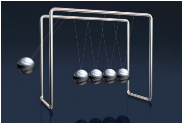
Figur 5.11: Newtons pendel
